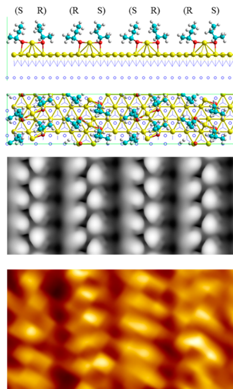
Figure 4. SAMs from a racemic mixture of the 2-butanethiols on Au(111) showing 4 \times 4 surface cells: (top) simulated STM image at 0 K and associated atomic structure of (SR)(RS) chirality, and (bottom) observed image for the (8 \times \sqrt{3})-4 phase; sulfur (red), carbon (cyan), hydrogen (white), gold top layer and adatoms (yellow), gold subsurface layer (blue bond to top layer), gold third layer (blue open circles), gold fourth layer not shown.
