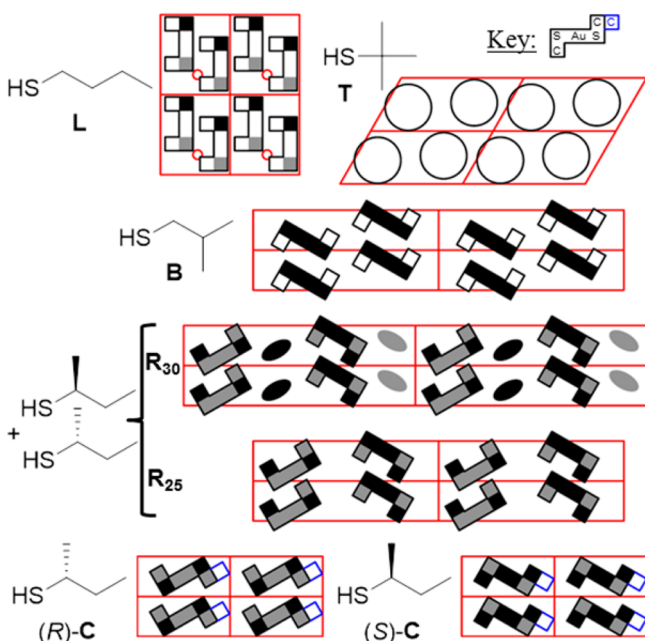
Figure 5. Sketches of four replicas of the surface cells of single domains within the butanethiol SAMs on Au(111), see Table 1. Black square and rectangular shapes depict the structure and chirality of C–S–Au–S–C units (see key), while circular and elliptical shapes depict adsorbates directly bound to Au(111) and blue squares indicate horizontally oriented ethyl groups. Shaded regions indicate either R (gray), S (black), or achiral (white) carbon, sulfur, or gold-adatom centers. Red circles indicate local vacancies.
