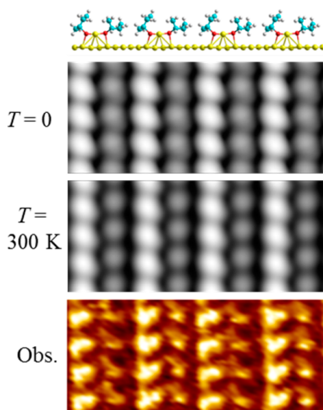
Figure 3. SAM of (R)-2-butanethiol on Au(111) showing a 4 \times 4 grid of (4 \times \sqrt{3})-2 surface cells: (top) simulated STM image at 0 K and associated atomic structure R_{ud} , (middle) simulated STM image for R_{ud} following 10 ps MD at 300 K, and (bottom) observed image; sulfur (red), carbon (cyan), hydrogen (white), gold (yellow).
