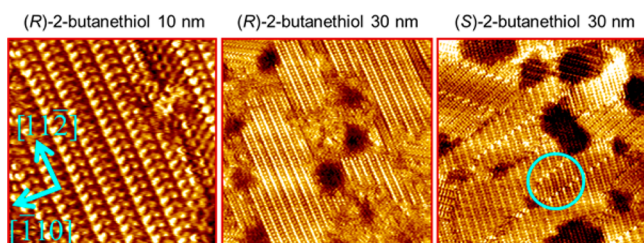
Figure 1. STM images of SAMs of chemisorbed ( R )-2-butanethiol (tunneling current I_t = 0.04 nA, bias voltage V_{\text{bias}} = 0.10 V) and ( S )-2-butanethiol ( I_t = 0.08 nA and V_{\text{bias}} = 0.40 V). The blue circle highlights two domain boundaries.
